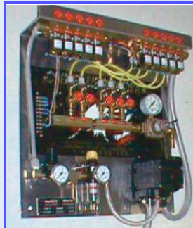
5 Bay Foaming Presoak Panel.
