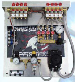
4 Bay Foam Brush Panel with Solenoids for Self-Serve Locations (shown with optional weep)
