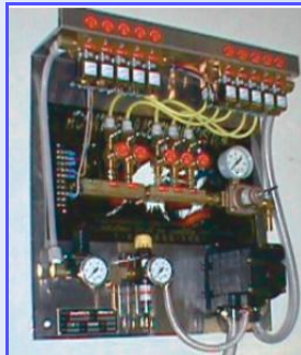
5 Bay Foaming Presoak Panel. Above picture shown with optional weep.
