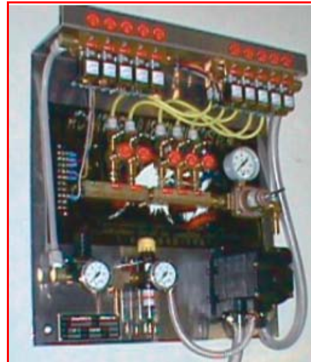
5 Bay Foam Brush Panel.
