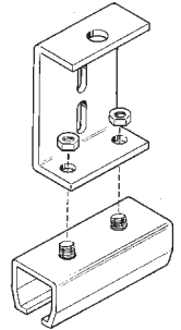
Universal Track Connector® Part HW100
